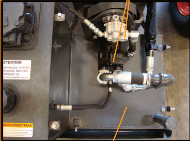
Front-mounted oil reservoir for greater visibility
